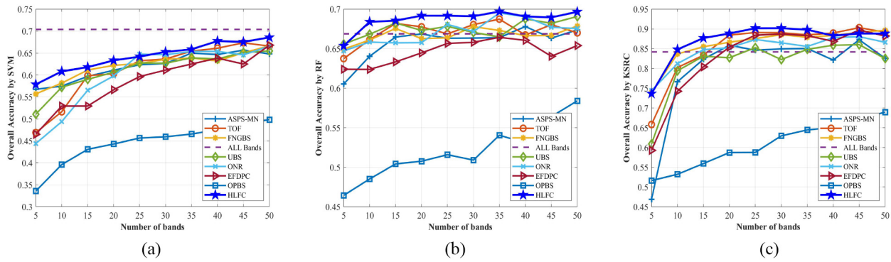
Fig. 4. OA of all competitors on the KSC dataset. (a) KSC-SVM. (b) KSC-RF. (c) KSC-KSRC.
