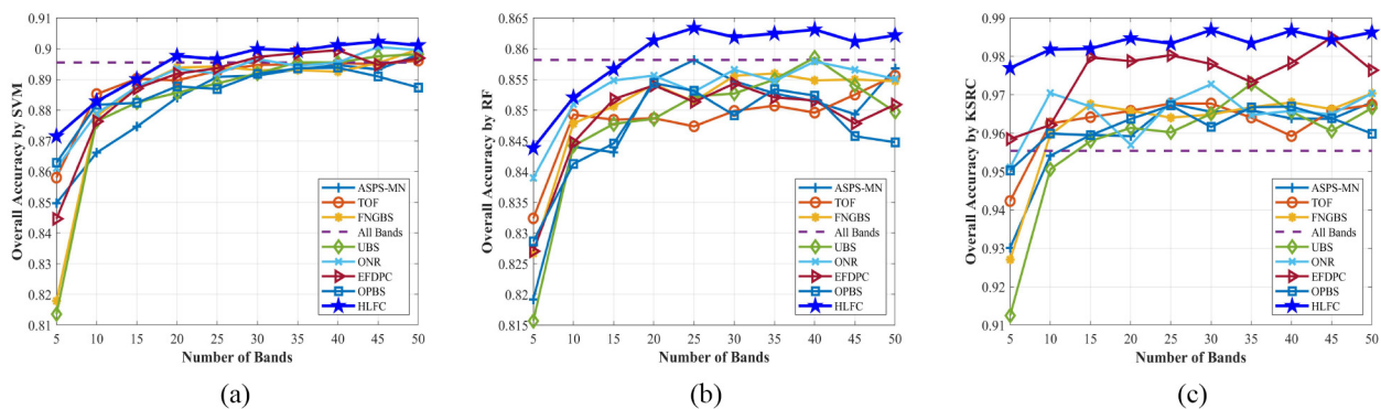
Fig. 6. OA of all competitors on the Salinas dataset. (a) Salinas-SVM. (b) Salinas-RF. (c) Salinas-KSRC.
