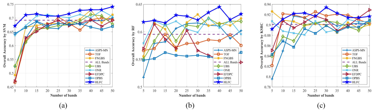
Fig. 5. OA of all competitors on the Botswana dataset. (a) Botswana-SVM. (b) Botswana-RF. (c) Botswana-KSRC.
